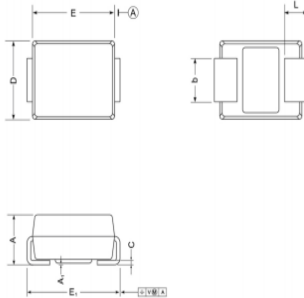
SMB mechanical data
